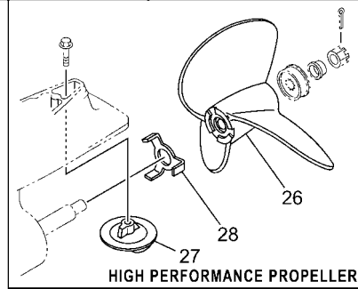
HIGH PERFORMANCE PROPELLER
