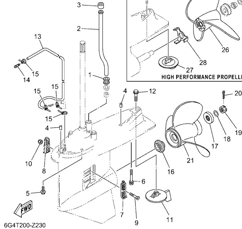
SDS PROPELLER 3 BLADE
